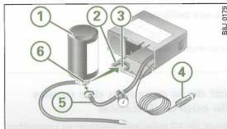
Fig. 167 Composants du Tire Mobility System
