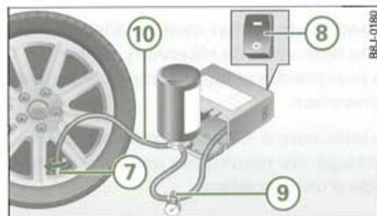
Fig. 168 Raccordement du Tire Mobility System
